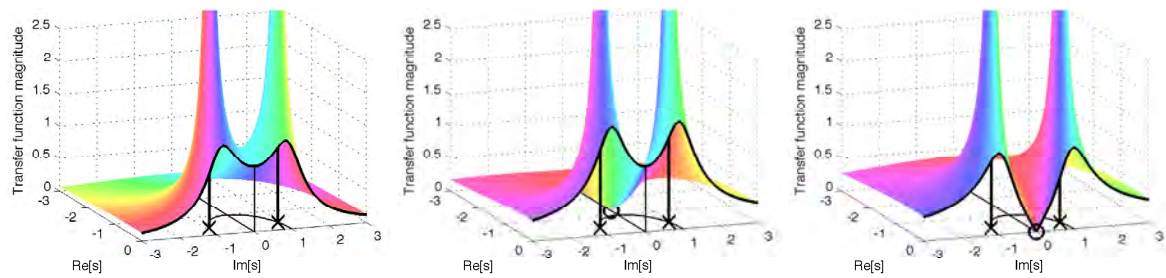
Figure 8.5: The transfer functions of the resonator filters A, B, and C, for natural frequency 1 and damping factor 0.4.
