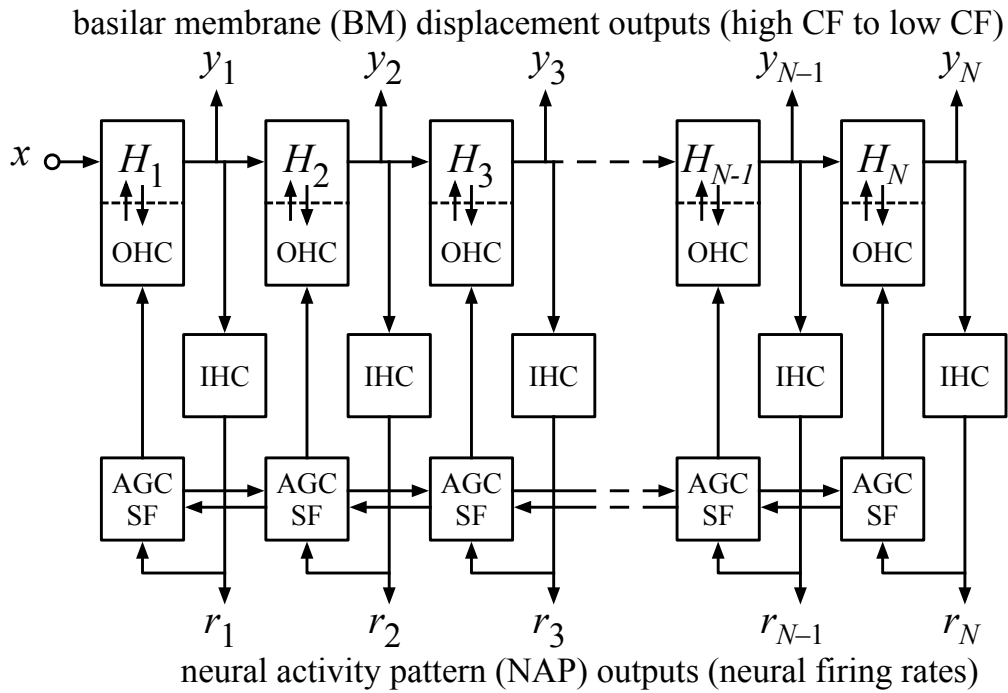
Figure 15.2: The Cascade of Asymmetric Resonators consists of the not-quite-linear transfer functions H_1 through H_N that model BM motion based on the cascade structure of Figure 12.9. Fast-Acting Compression is implemented by the other elements, including the OHC model that is tightly integrated with the filter stages and gives them their nonlinearity, and the coupled AGC smoothing filters (AGC SF) that modulate how the OHCs control the parameters of the filters. Between these main parts is a detection nonlinearity, such as an IHC model, which can have some compression and adaptive state of its own. The lateral interconnections of the smoothing filters allow a diffusion-like smoothing, or coupling, across both space and time. Outputs from the CARFAC include BM motion y_i (a set of compressed nearly-linear filterbank outputs) and an estimate of average instantaneous auditory nerve firing rate r_i , the NAP.
