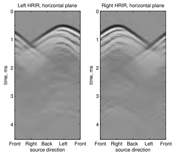
Figure 22.5: Head-related impulse responses of a dummy head, for sounds from various directions in the horizontal plane. The impulse responses are mapped to gray levels and displayed from top to bottom, from an arbitrary time origin shortly before the arrival of a sound impulse at the head; the x axis represents the azimuth angle of the sound source. Separate arrivals can be seen when the sound goes around the front and back of the head as in the left ear when the sound is from the right. For a sound from an intermediate azimuth (not a multiple of 90 degrees), differences in pinna echoes, the ridges near the top of the plot, help distinguish front from back.
