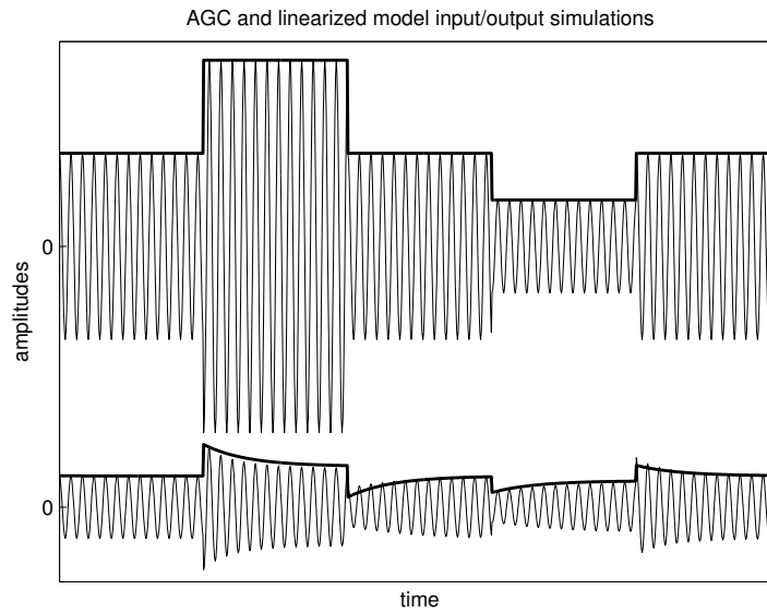
Figure 11.9: Inputs (top) and outputs (bottom) of a simulation of the multiplicative AGC system of Figure 11.2, and its small-signal linear model (see Figure 11.10 for parameters), as the input amplitude is stepped up and down by factors of 2. The amplitude-modulated sinusoids are the inputs and outputs of the nonlinear AGC simulation, while the bold curves are the inputs and outputs of the linearized model added to the equilibrium levels, scaled up by a factor of \pi for comparison to the peaks of the sinusoids. The fact that the output curves do not perfectly match is an indication that the linearization about the equilibrium condition is not a perfect model of the nonlinear dynamics. The equilibrium gain from input to output is g_{\text{eq}}H = 0.34 , which is why the output curves are so much smaller than the input curves.
