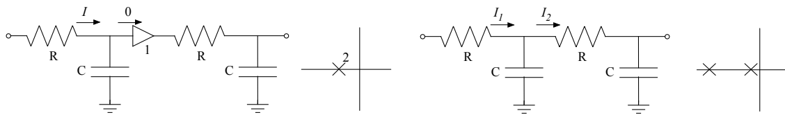
Figure 6.12: A cascade of two identical RC filters separated by a buffer amplifier (left) and without a buffer (right). The buffer (triangle with label “1” indicating its gain), takes zero input current and copies its input voltage to its output, so the second filter stage does not influence the first stage by taking current out of it, or “loading” it. The resulting transfer function H^2 , the square of the one-pole stage transfer function, has two poles in the same location, at s = -1/RC , as shown in the left pole plot. Without the buffer, some of the current through the first resistor flows into the second, contrary to what we assumed when we computed the transfer function of the RC filter. Such mutual coupling—the second stage affecting the first stage—results in a different filter, with two different pole locations as shown in the right pole plot.
