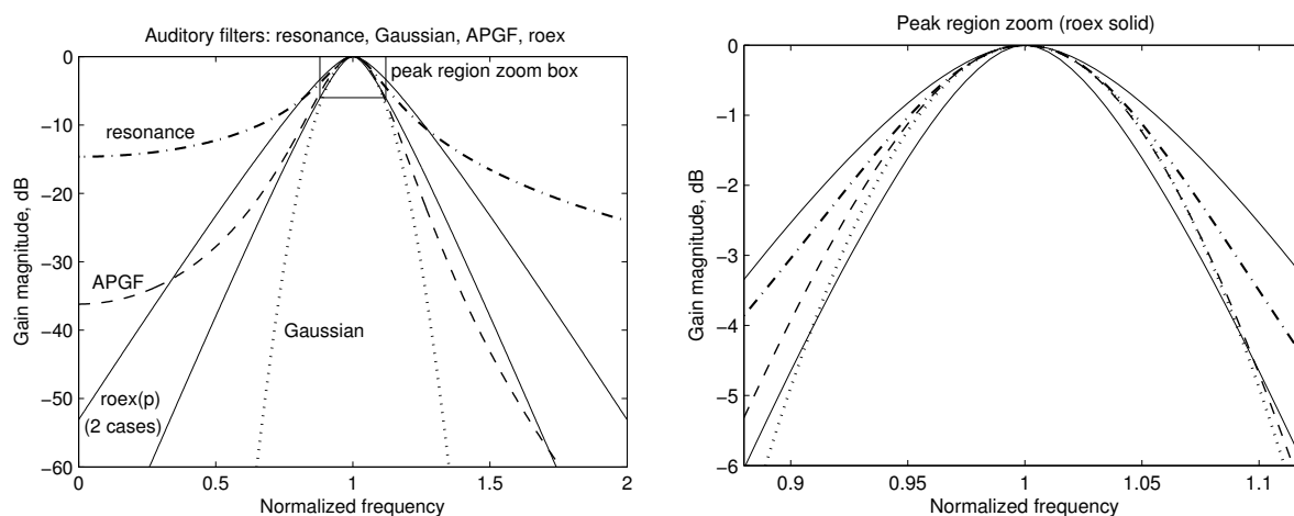
Figure 13.1: A few auditory filter model shapes, showing the large room for possibilities between the simple two-pole resonator and the Gaussian filter. The asymmetric 4th-order all-pole gammatone (APGF), and the symmetric roex(p) are included as examples of intermediate shapes. The illustrated filter shapes are matched for equal curvature at the peak, except for the sharper roex(p) case. The peak region zoom on the right shows how the matched roex peak curvature leads to rather wide skirts, and more reasonable skirts lead to a rather sharply curved peak, compared to the other filter shapes.
