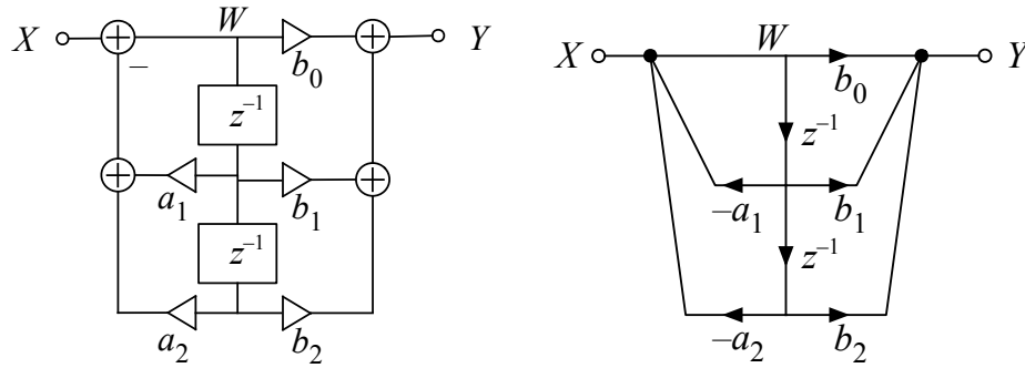
Figure 7.8: In a typical representation of a direct form II discrete-time or digital second-order section (left), the feedback block that makes the poles comes first, followed by the feed-forward block that makes the zeros. These blocks share two delay elements, delaying an intermediate signal, neither X nor Y , which is the output of the first block and the input of the second block. The directions of signal flow are implied by the coefficient multipliers (the oriented triangles), so the generous use of arrows that we saw in Figure 7.5 is typically avoided. In the even more concise form (right) arrows on lines are used to indicate multiplicative operators, including the delays, and dots represent additions.
