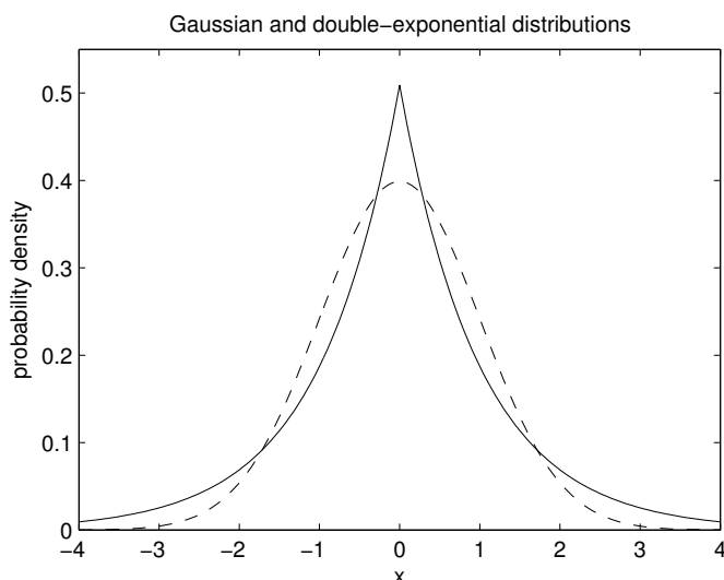
Figure 24.12: Gaussian (dashed curve) and double-exponential (solid curve) prior distributions on parameters, compared here with variances equal to 1, correspond to using L2 and L1 regularizers, respectively. The double-exponential distribution has many more values at zero, fewer small nonzero values, and more large values, compared to the Gaussian.
