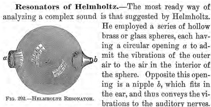
Figure 8.2: Before we had electrical resonators, fluid-mechanical Helmholtz resonators were used for sound analysis. Helmholtz developed and used a set of these resonators, tuned to the frequencies of musical notes, to help him “hear out” the sinusoidal components of complex tones. These resonators are tuned by the interaction of the springiness of the air in the globe with the momentum of the mass of air in the neck. Figure from Quackenbos et al. (1891).
