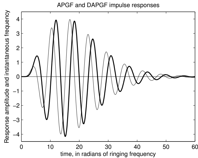
Figure 9.7: Impulse responses of the 4th-order all-pole gammatone filter (APGF, heavy curve) and its derivative, the DAPGF (light curve), with pole damping \zeta = 0.2 ( Q = 2.5 , Q_{3\text{dB}} \approx 5 ).
