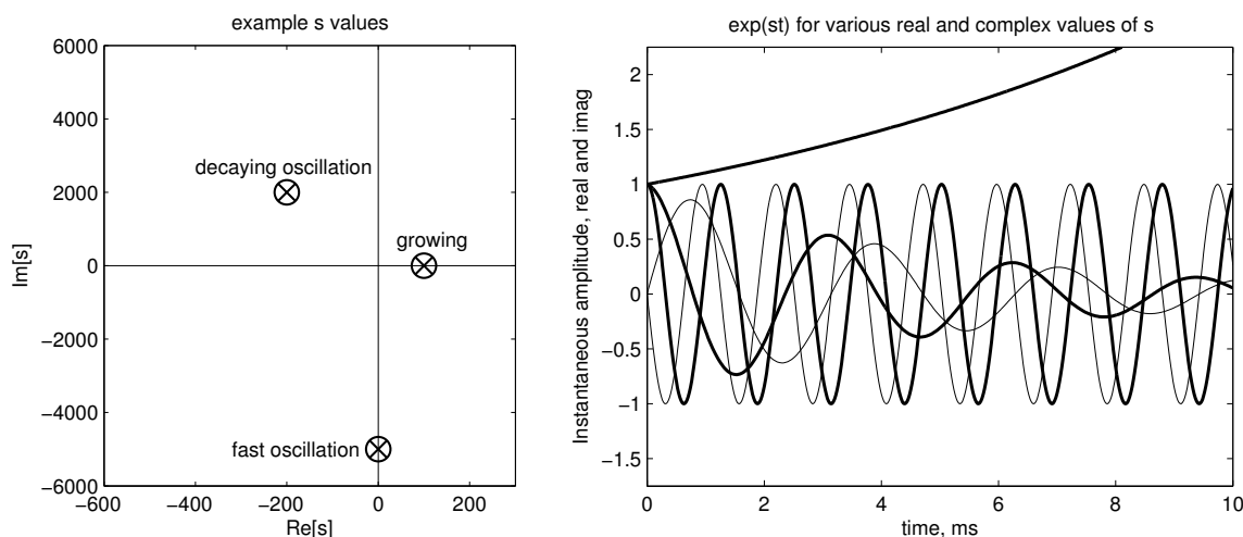
Figure 6.5: Plots of example s values (left) and the real and imaginary parts of \exp(st) (right); for complex s , the imaginary part is shown by light curves, and the real parts are always heavy curves. One real s value, s = 100 , yields the slow exponentially growing curve on top. A pure imaginary value s = -i5000 corresponds to the steady high-frequency sinusoids shown; notice that the imaginary part leads the real part, since this one is a negative frequency complex sinusoid. The damped sinusoid shown corresponds to s = -200 + i2000 . In each case, the units of s are inverse seconds, or radians per second. If the input to a linear time-invariant system, or filter, is any of these signal shapes, then the output will be the same, just multiplied by the complex factor H(s) for that filter at that s value. That is, these functions \exp(st) are eigenfunctions of all LTI systems (subject to some region-of-convergence restrictions that we mostly ignore).
