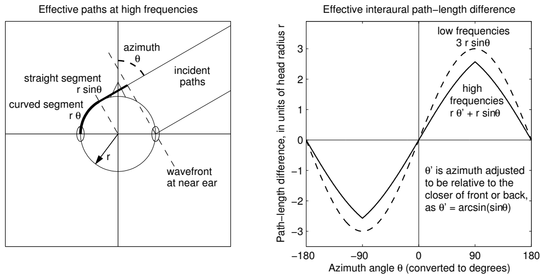
Figure 22.4: High-frequency sounds follow the shortest path around the head. In the horizontal plane, for sounds incident from an azimuth angle of \theta , the extra path length to the far ear is r\theta + r \sin \theta (using the azimuth angle modified as shown to be an angle of magnitude less than 90 degrees in the interaural-polar system). Due to diffraction effects, low-frequency sounds experience a somewhat larger time lag than this estimate would suggest; about 50% larger for small angles (Kuhn, 1977). The angle illustrated on the left is on the +60 degree cone of confusion shown in Figure 22.3.
