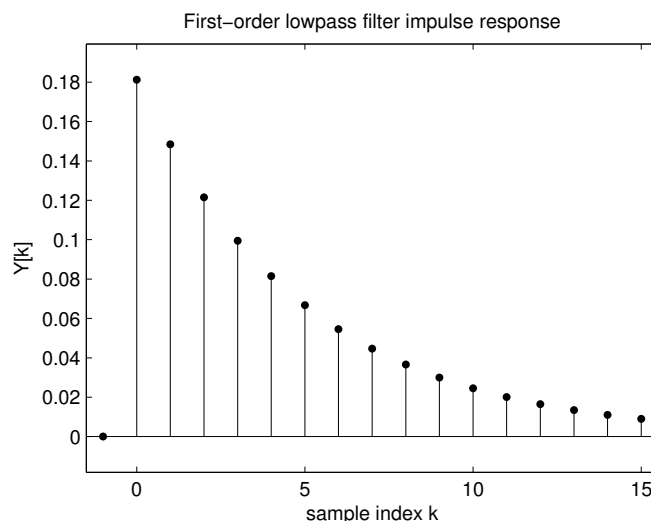
Figure 7.7: The discrete-time first-order smoothing filter’s impulse response is a geometric sequence (for k \geq 0 ), a sequence of samples of an exponential decay.
