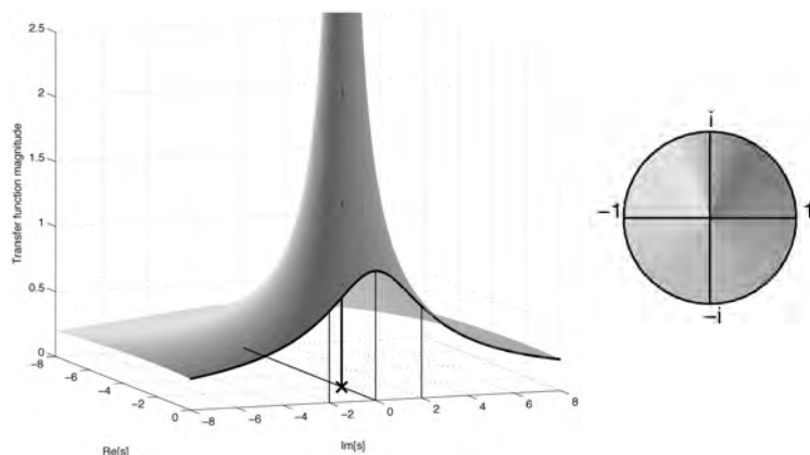
Figure 6.4: The transfer function of the example RC filter of Figure 6.1. The magnitude of H(s) is plotted as a surface height above the complex s plane, while the phase of H(s) determines the hue of the surface color (following the phase–hue legend on the right; see color plates). For the example filter with \tau = 0.5 , the transfer function has a singularity at s = -2 + i0 (at cross and heavy vertical line). The surface is cut along the imaginary s axis to reveal the frequency response. The frequencies \omega = 0 (DC) and \omega = \pm 2 (the 3-dB points) are marked by lines.
