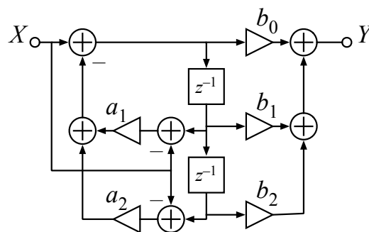
Figure 8.19: The two-pole filter of Figure 8.18 is easily modified to include zeros. In this form, the poles can be moved, while the zeros are held fixed, without the DC gain changing. The relationship of coefficient values to pole and zero locations is as discussed in Section 7.11, except that pole-location-dependent numerator of the A factor there is subsumed in the input gain 1 + a_1 + a_2 provided by the way the input is connected here.
