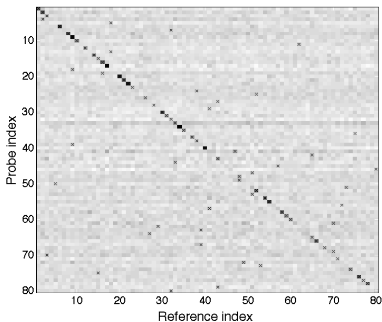
Figure 27.7: Scores matrix for comparing all probes and references in the dataset. Darker pixels denote higher scores, indicating a more likely match. Black crosses denote the best-matching reference for each probe.
