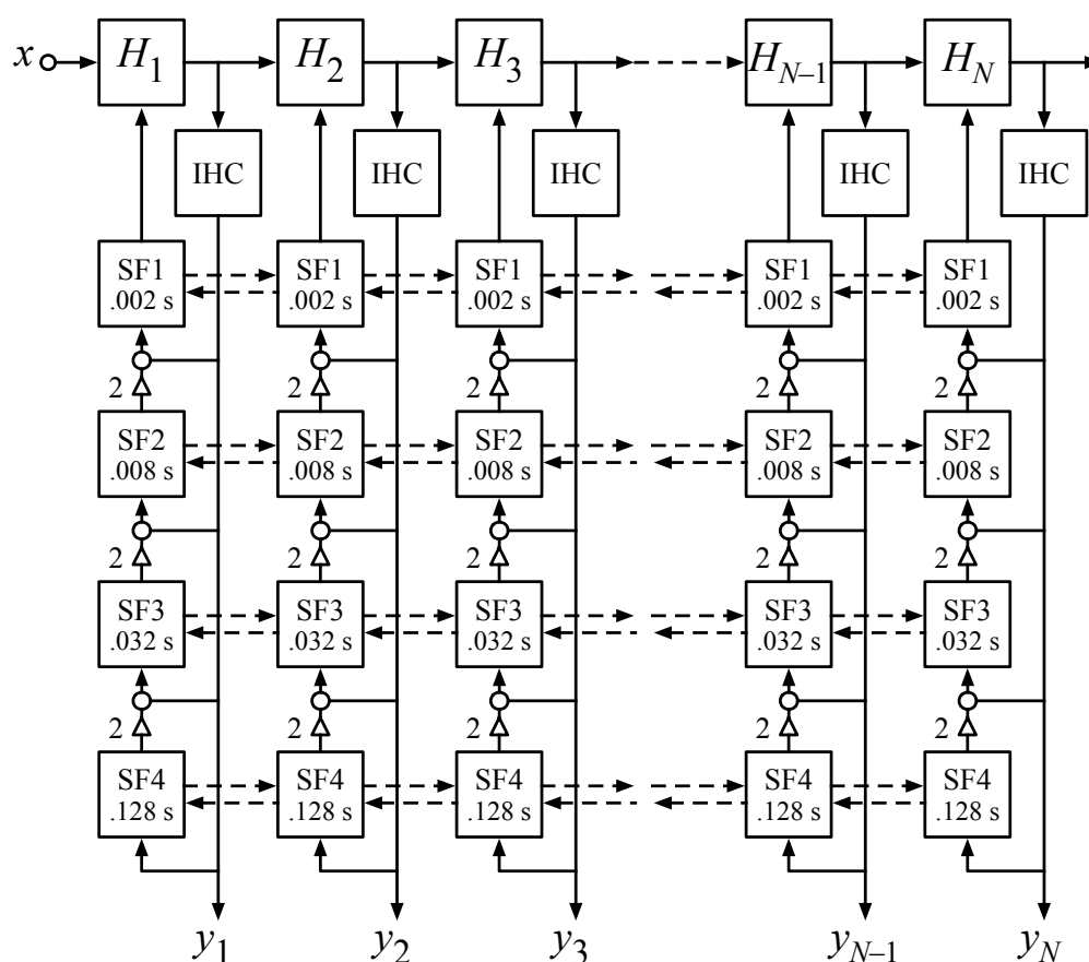
Figure 19.5: The filters in each AGC channel are based on the parallel-of-cascades version in Figure 19.1. In this configuration, the faster filters define a shorter (more local) loop, and it is easier to run the more-remote slower filters at lower sample rates, since their output steps will be smoothed by other filters before being applied to control the CAR filter stage damping. Neglecting the sampling approximations, the loop-filter transfer functions are as shown on the right in Figure 19.4. The lateral interconnections are shown dashed; the mechanism for spatial cross-coupling is detailed in the next figure.
