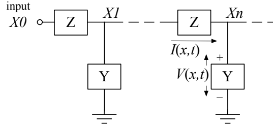
Figure 12.4: The general transmission-line model uses series impedances Z proportional to the distributed line's series impedance per unit length, and shunt admittances Y proportional to the line's shunt admittance per unit length. The electrical signals used to analyze it are the currents through the series elements and voltages across the shunt elements, signed as shown. The elements Z and Y are more general than the inductors and capacitors of Figure 12.2; each may contain series or parallel connections of several lumped elements, for example.
