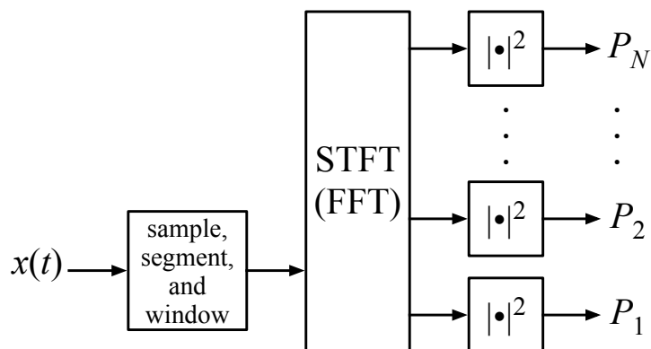
Figure 5.2: The short-time spectrum of a signal x(t) can be estimated by a short-time Fourier transform (STFT, typically using the fast Fourier transform algorithm, FFT). The center frequencies are in arithmetic progression, and the bandwidths all equal, unless a further stage of channel combining is added. A segment length and window function establish the time scale of the STFT. The power outputs from such an analysis are typically next compressed through a logarithmic or power-law function.
