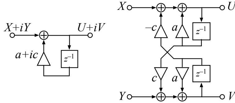
Figure 8.20: A one-pole complex-valued filter (left) is equivalent to the real-valued two-pole filter known as a coupled-form filter (right), if X , Y , U , and V are real, as is evident by expanding the complex multiplication into its four real terms. The system on the right can be viewed as a complex system with one pole at z_p = a + ic , or as a two-input–two-output linear system with real outputs whenever both inputs are real. The two-input–two-output system can nevertheless be analyzed like other LTI systems in terms of complex inputs, outputs, and eigenfunctions. If the input to the complex system on the left is real, then that system is equivalent to the one on right with the Y port unused (zero imaginary part). For that one-input system, taking only the real-part output, U , gives two poles, at z_p and z_p^* , and one real zero at z_z = a (and a zero at z = 0 that keeps it minimum-phase). Similarly, the transfer function from the X input to the real V output has only the pole pair (and the zero at z = 0 ), as can be verified with a little algebra.
