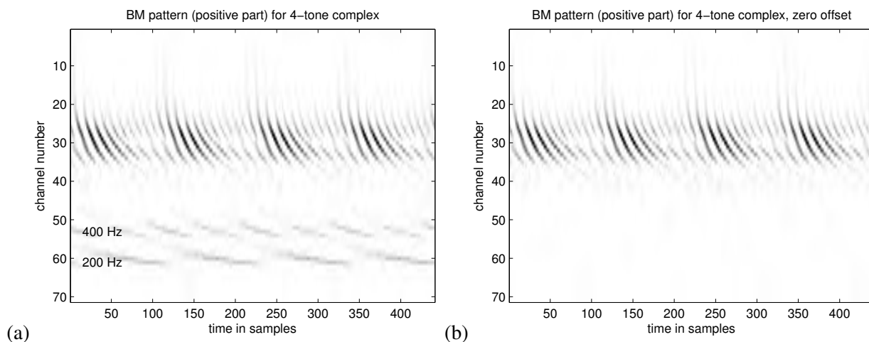
Figure 17.6: These cochleagrams show the positive part of the BM motion (filter outputs) for the 4-tone complex stimulus at 60 dB SPL, the level at which the relative amounts of 200 Hz and 400 Hz quadratic distortion tones is highest with the default NLF offset parameter. The left (a) image is for the default CARFAC, and the right (b) is with zero offset in the NLF. The 20 ms segment encompasses four cycles of the 200 Hz missing fundamental. The relatively small offset asymmetry shown in Figure 17.2 and Figure 17.5 is enough to cause relatively large QDTs.
