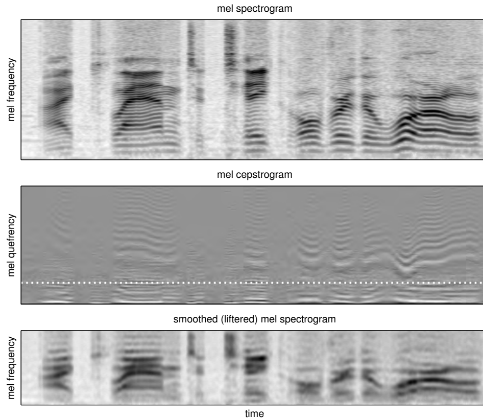
Figure 5.10: Mel-scale power-law spectrogram (top), mel-frequency cepstrogram or MFCCs (middle), and liftered mel spectrogram (bottom) reconstructed from the low-quefrency cepstral coefficients (from below the dotted white line); though this low-quefrency region looks bigger than in Figure 5.9, it is only 22 coefficients instead of the 33 used in the linear-frequency case. The mel frequency warping interferes with the usual cepstrum's simple representation of periodicity in the high-quefrency region, smearing out the pitch curve into ripples, but gives a much better distribution of spectral information.
