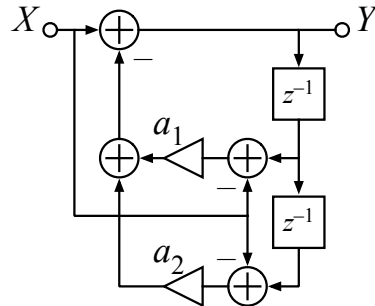
Figure 8.18: A direct-form two-pole filter stage with the input connected as shown here has unity gain at DC. It is evident by inspection that if the input is constant and the output is equal to the input, then the subtracted feedback will be zero, no matter what the coefficient values a_1 and a_2 are, due to the differences being zero where the input is subtracted from the two delayed outputs; therefore output equal to constant input is an equilibrium point, so the DC gain is 1. The transfer function to Y as shown also has two zeros at z = 0 , and is a minimum-phase transfer function (assuming the poles are inside the unit circle, making it stable); an output taken after one or both of the z^{-1} delay elements has one or two samples of extra delay, canceling one or both zeros, so would not be minimum phase.
