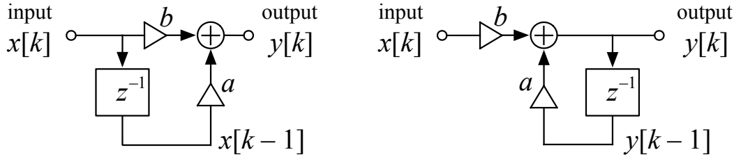
Figure 7.1: The signal-flow diagrams of two different first-order digital filters are shown here: a finite-impulse-response (FIR), or nonrecursive, filter on the left, and an infinite-impulse-response (IIR), or recursive, filter on the right. With appropriate choice of coefficients a and b , namely a = 1 - b , with both coefficients between 0 and 1, these are smoothing filters (that is, they suppress fluctuations and have average output equal to average input). The FIR filter on the left can only do a little bit of very local smoothing, while the IIR filter on the right behaves like the RC lowpass filter, with potentially very long time constant, when the coefficients make it a smoothing filter. The label z^{-1} in the box represents the unit delay operator. The triangles represent multiplication by the constant coefficients shown. The two filters' difference equations, y[k] = bx[k] + ax[k-1] and y[k] = bx[k] + ay[k-1] , and z -domain operator equations, Y = bX + z^{-1}aX and Y = bX + z^{-1}aY , are apparent from the signal-flow diagrams. Labeling the input x[k] and the output y[k] as here suggests the operation steps on sequences of samples, with z^{-1} being a unit delay, or memory element. We alternatively label them X and Y , which suggests interpreting the z^{-1} as a transform operator. We switch back and forth between such labels and interpretations, as we did in Chapter 6.
