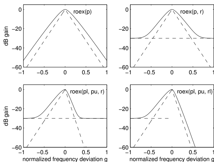
Figure 13.2: The roex family can take various parameters, including some illustrated here. In the \text{roex}(p) model (upper left), the factor 1 + p|g| rounds the filter’s power gain above a symmetric triangular skeleton. In the \text{roex}(p, r) model (upper right), a floor at gain r is imposed (here at r = 0.001 ). In the \text{roex}(pl, pu, r) model (lower left), the upper and lower sides have different slopes, but the same floor. Allowing separate floor levels, or using no floor on the upper side, as Rosen and Baker (1994) did, allows more realistic asymmetric filter shapes (lower right) (we do not treat this as a separate model here, just a different parameterization of the asymmetric version). All of these are still too peaky (not rounded enough) near the peak, compared to more realistic models.
