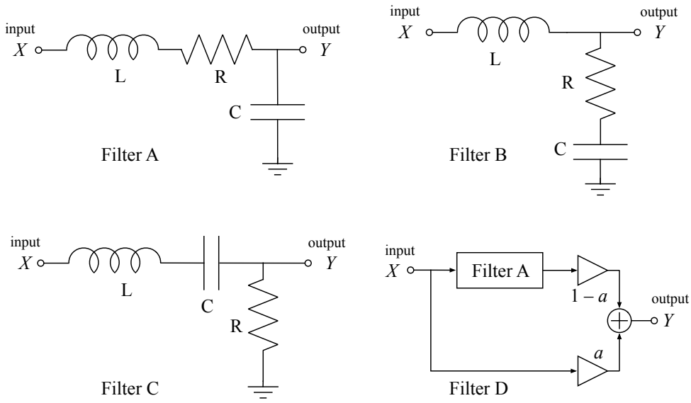
Figure 8.3: Circuit diagrams of four resonant filters. Filter A (top left) is the same as previously shown in Figure 6.9. Filter B (top right) has the resistor, the energy-dissipating element, moved from the series impedance (the impedance of the elements connecting the input to the output in the voltage divider circuit) into the shunt impedance (the impedance of the elements connecting the output to ground). Like Filter A, Filter B has unity gain at DC, since the DC impedance of the capacitor in the shunt leg is infinite. Filter C (bottom left) is a second-order filter with capacitive coupling, or zero response at DC (at zero frequency), since the capacitor is now in series. Filter D (bottom right) uses a pair of adjustable-gain buffer amplifiers (shown as triangles) to mix the output of a filter A circuit with its input. All of these filters have the same pair of poles, and all are relevant as basic building blocks and limiting cases in our study of auditory filters in subsequent chapters.
