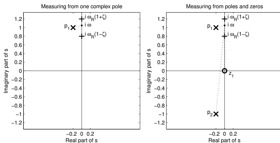
Figure 8.11: Graphical construction of the frequency responses of resonators. Using the left-hand plot with a single complex pole, the gain magnitude of the universal resonance curve, or of the one-pole complex resonator, is inversely proportional to the distance between the pole p_1 and the frequency point i\omega (as a function of \omega ), here illustrated for \omega just above the ringing frequency, \omega_R . Frequencies are scaled such that \omega_R = 1 . The cross marks “+” at i\omega_R(1 \pm \zeta) indicate the points where the distance from the pole to the frequency point increases by \sqrt{2} (the 3-dB points, deviations g = \pm 1 in the universal resonance curve, also marked by “+” in Figure 8.10). The real filters have a second pole, p_2 ; and may have a zero, z_1 , as shown in the right plot. The relative distance to the second pole doesn’t vary much near the resonance peak, but does move and tip the peak of Filter A a bit when it is included. For filter C, there is also a zero at s = 0 ; the distance to the zero appears in the numerator, so moves and tips the response in the opposite direction. The pole and zero positions shown represent \zeta = 0.2 or Q = 2.5 , corresponding to the curves in Figure 8.10, where DC is at g = -5 . Pole-zero plots such as these were once commonly used for measurement and calculation of frequency responses, but with modern computers we no longer need such aids; on the other hand, they are still very useful as tools to suggest at a glance the form of the transfer function surfaces of Figure 8.5.
