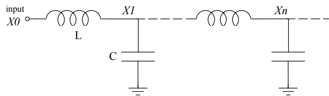
Figure 12.2: Waves travel at speeds somewhat less than the speed of light along wire transmission lines, including telephone lines, coaxial cables, power lines, etc. Such lines can be approximated or modeled by LC delay lines, circuits of iterated lumped elements as shown here.
