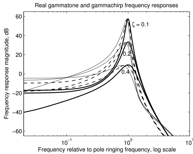
Figure 9.11: The Fourier transforms of the impulse responses are displayed here, for the three impulse responses of the previous figures, plus modifications with half and double damping values. The c = -1 gammachirp (dashed curves) has a nonmonotonic damping dependence in the tail, as a zero happens to move close to s = 0 when the damping is reduced. In several cases shown, a zero moves to near s = 0 , pushing the low-frequency tail down; in some of the gammachirp cases, there's also a dip on the high side, due to another spurious zero that comes from interference between the complex gammachirp and its conjugate. These behaviors also have a complicated dependence on the \phi values used; here we use the same values as in Figure 9.9.
